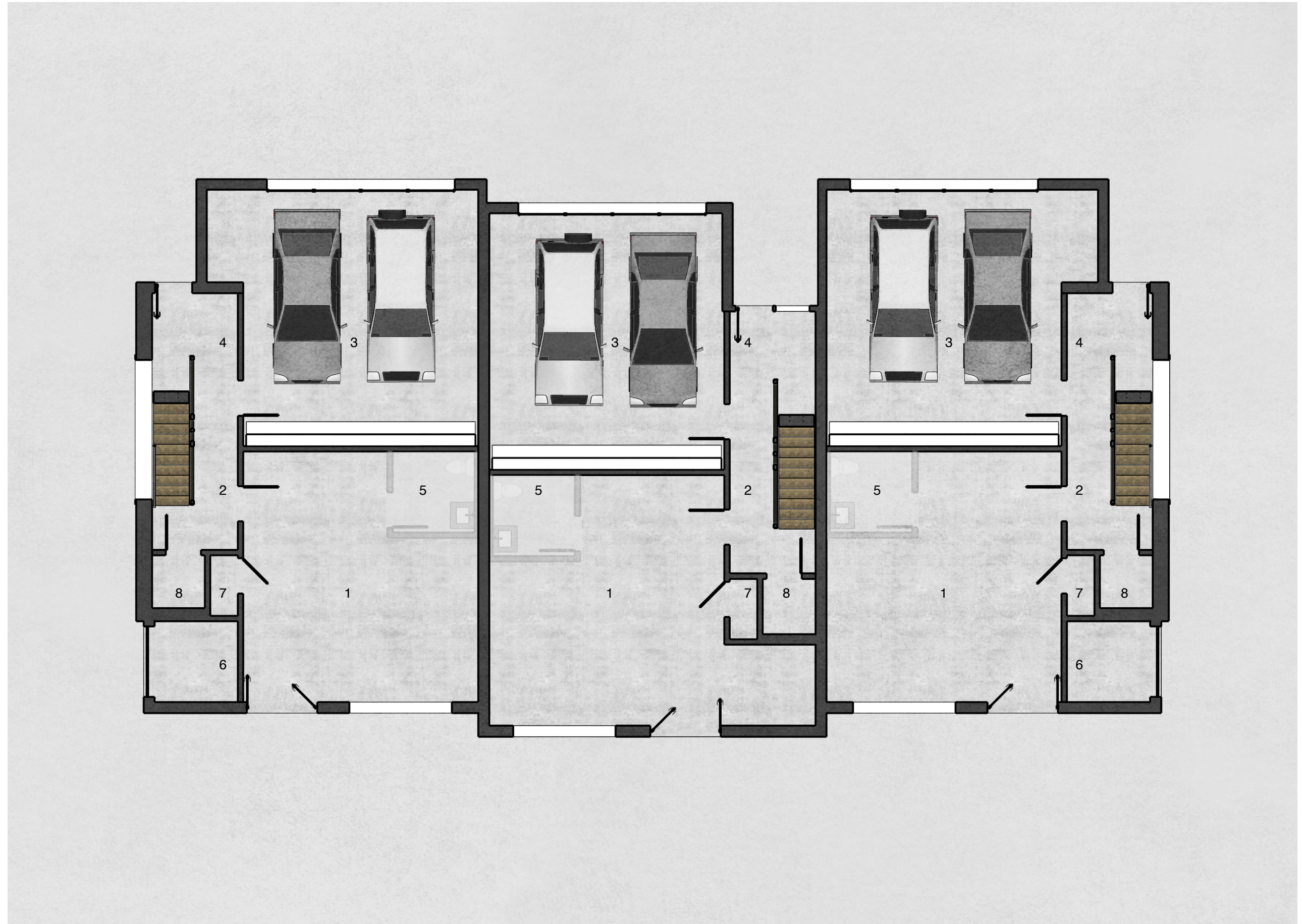
ground floor // 1 commercial 20 x 21 2 vestibule 7 x 5 3 garage 23 x 21 4 entry 7 x 16 5 bath 7 x 7 (future) 6 mechanical room (common) 7 closet 8 elevator (future)
